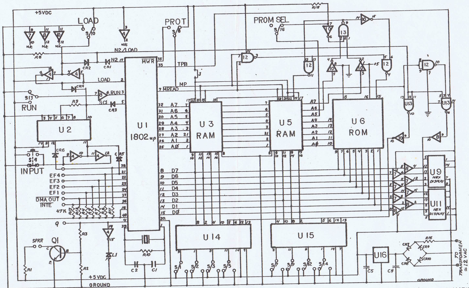
COSMAC SCHEMATIC REV 2.1
